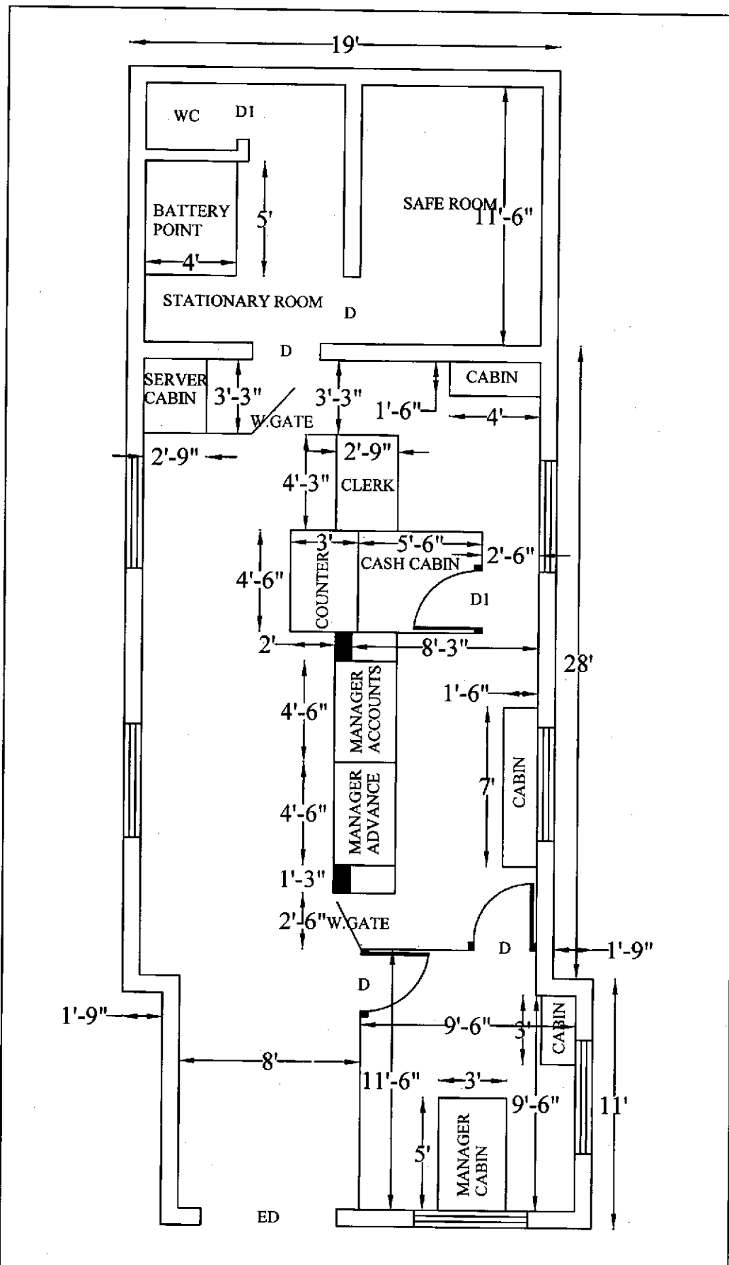
INTERIOR PLAN FOR KAVERI GRAMEENA BANK PREMISES AT ARUDI BRANCH, BANGALORE NORTH TALUK.
